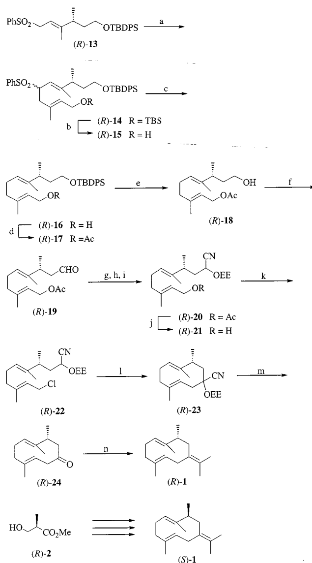
Scheme 3. Synthesis of the enantiomers of 9-methylgermacrene-B ( 1 ); reagents: (a) n BuLi, THF, HMPA, then 4 (88%); (b) AcOH, THF, H 2 O (85%); (c) LiEt 3 H, PdCl 2 (dppp), THF (82%); (d) Ac 2 O, C 5 H 5 N (98%); (e) n Bu 4 NF, THF (90%); (f) Dess–Martin periodinane, CH 2 Cl 2 (85%); (g) TMSCN, KCN-18-crown-6; (h) BnNMe 3 F, THF, H 2 O; (i) EtOCH=CH 2 , TsOH, C 6 H 6 (quant.); (j) K 2 CO 3 , MeOH (89%); (k) MsCl, LiCl, DMF, s -collidine (95%); (l) NaHMDS, THF (47%); (m) PPTS, MeOH, then NaOHaq, Et 2 O (57%); (n) CBr 2 Me 2 , Sm, SmI 2 , CrCl 3 , THF (60%)
