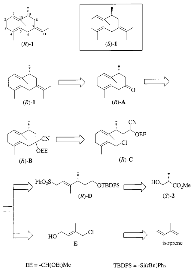
Scheme 1. Structures of the enantiomers of 9-methylgermacrene-B ( 1 ) and the retrosynthetic analysis of ( R )- 1
