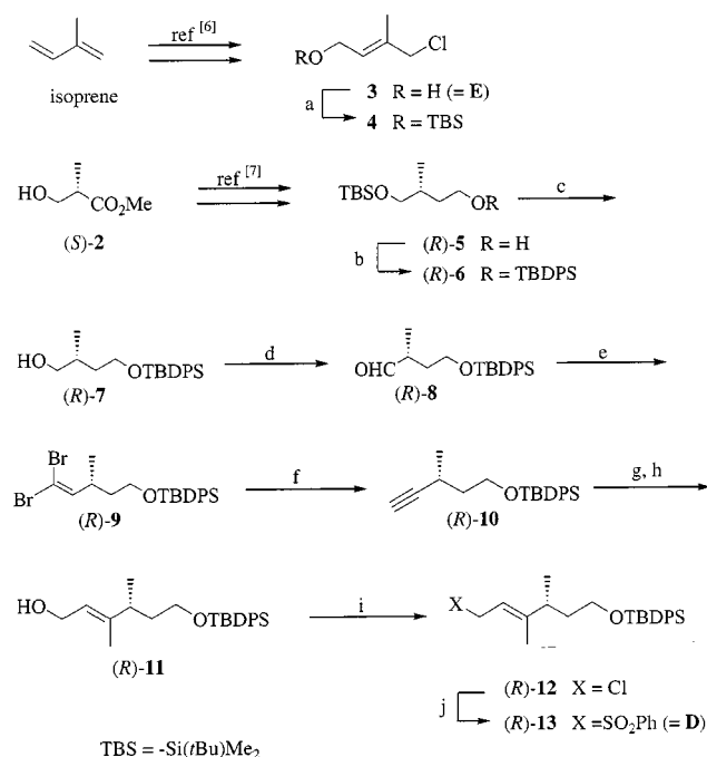
Scheme 2. Synthesis of the two building blocks 4 and ( R )- 13 ; reagents: (a) TBSCl, imidazole, DMF (quant.); (b) TBDPSCl, imidazole, DMF (89%); (c) AcOH, THF, H 2 O (84%); (d) (COCl) 2 , DMSO, Et 3 N, CH 2 Cl 2 ; (e) PPh 3 , CBr 4 , CH 2 Cl 2 [87% based on ( R )- 7 ]; (f) n BuLi, Et 2 O (98%); (g) Me 3 Al, Cp 2 ZrCl 2 , CH 2 Cl 2 , H 2 O; (h) i) n BuLi, hexane; ii) (CH 3 O) n , THF (85%); (i) PPh 3 , CCl 4 ; (j) PhSO 2 Na·2H 2 O, DMF [76% based on ( R )- 11 ]
